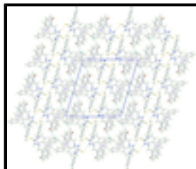
Fig. 2. A view in projection down the b axis of the crystal packing in (I) highlighting the mode of association between the constituent ions. The N—H...S, O—H...Cl and C—H...Cl interactions are shown as orange, blue and brown dashed lines, respectively.
