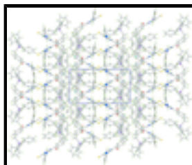
Fig. 3. A view in projection down the c axis of the crystal packing in (I) highlighting the stacking of layers along the a -direction. The N—H...S, O—H...Cl and C—H...Cl interactions are shown as orange, blue and brown dashed lines, respectively.
